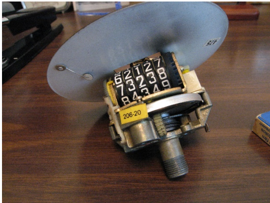
Figure 5 Speedo Internals
